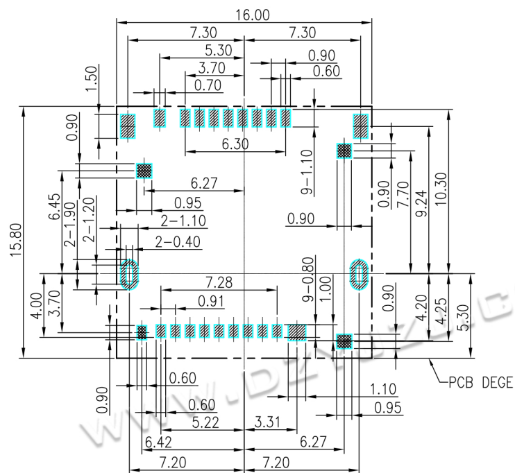
RECOMMENDED P.C.B LAYOUT TOP VIEW(TOLERANCE+/-0.05)
